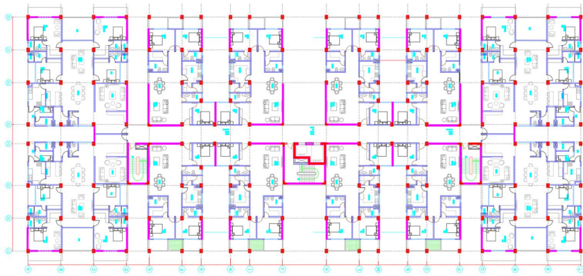
20-storey apartment in Bangladesh – Precast structure design
