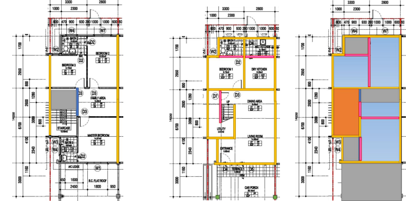
2-storey terrace house in Malaysia – Precast structure design
