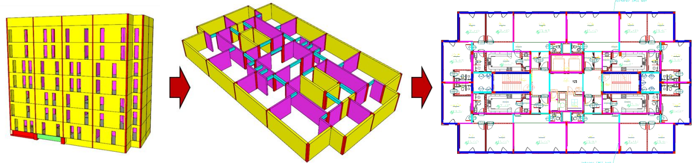
7-storey apartment in Saudi Arabia – Precast structure design
